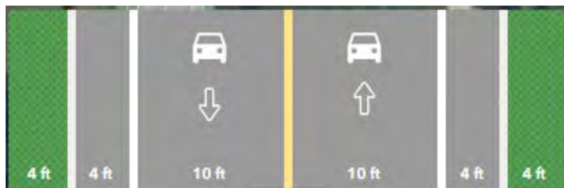
Figure 2: Five Mile Rd, Section near Solterra Cir
