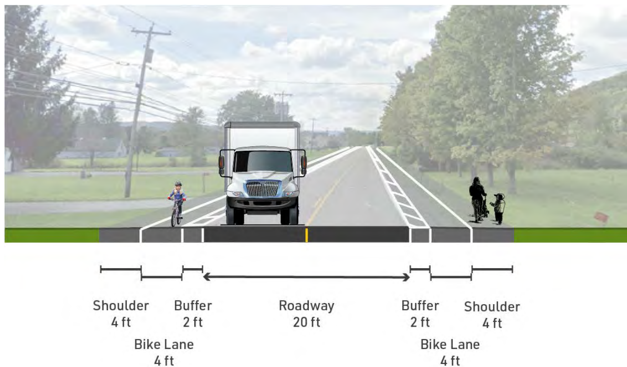
Figure 10. Paved Shoulders, Section View
