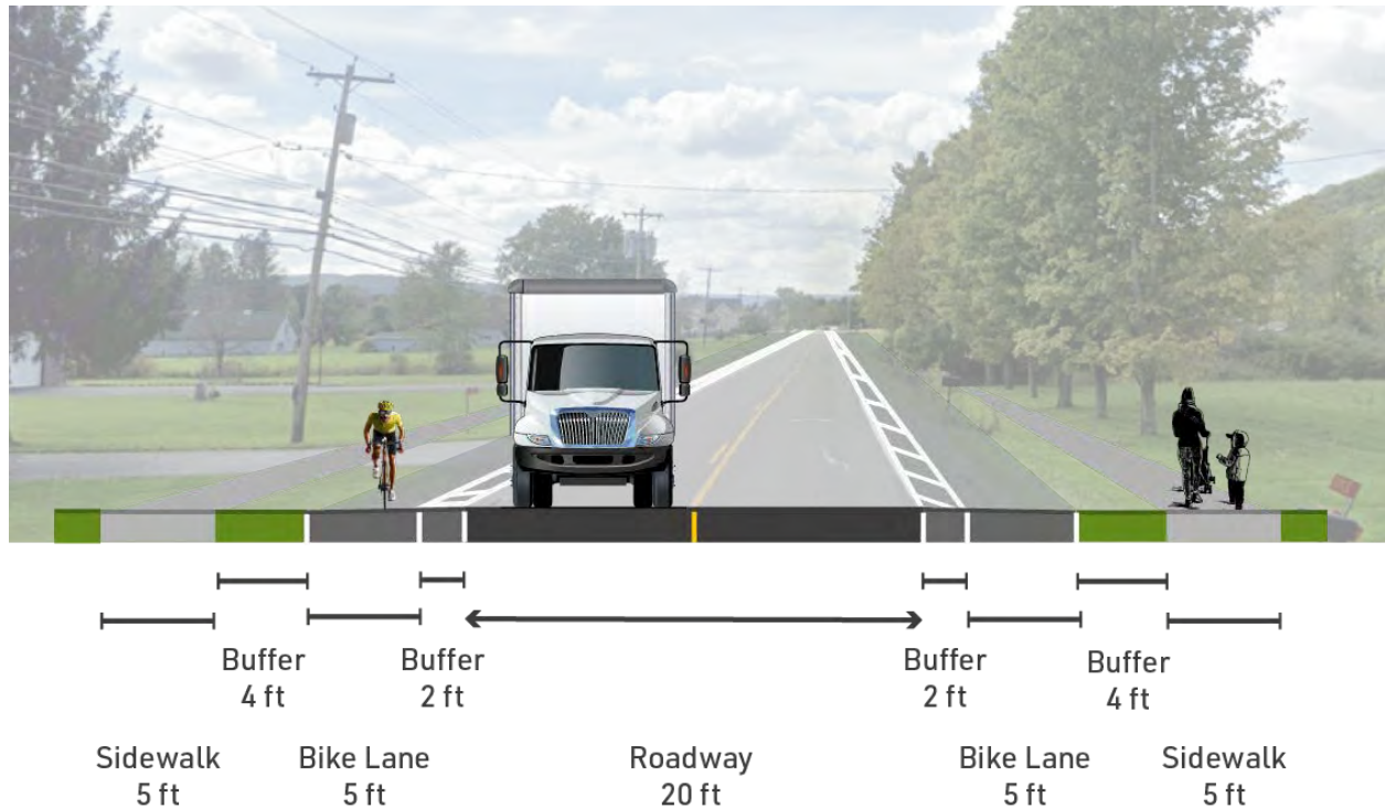
Figure 12. East Side Path, Section View
